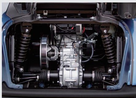
Performance tuned independent rear suspension (For QuietTech EFI model).
